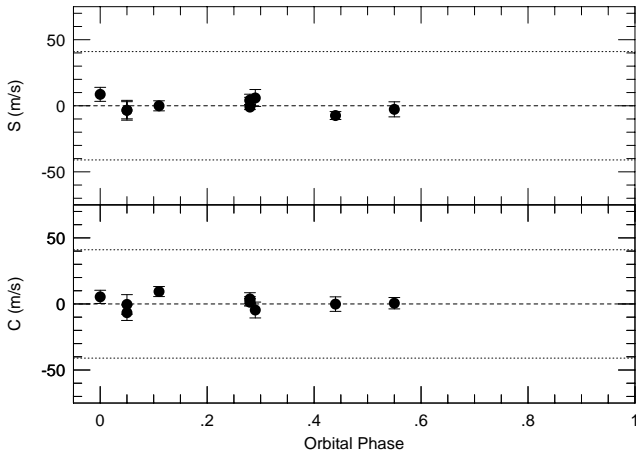
Fig. 6. The mean velocity span (top) and curvature (bottom) of the spectral line bisectors of \beta Gem as a function of orbital phase (590-day RV period). Dotted lines mark the maximum extent of the RV variations and the dashed line is the zero level.
