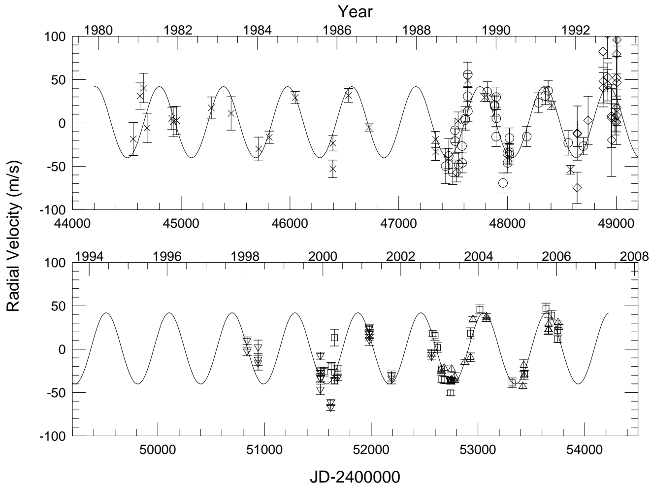
Fig. 1. Radial velocity measurements for \beta Gem from the 6 data sets: CFHT (crosses), DAO (diamonds), McD-2.1m (circles), McD-cs21 (inverted triangles), McD-MOPS (squares), and TOPS (triangles).
