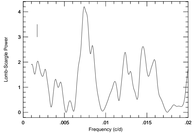
Fig. 7. The Lomb-Scargle periodogram of the Hipparcos photometry. The vertical line marks the orbital frequency.
