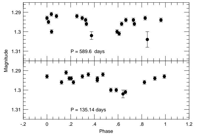
Fig. 8. The Hipparcos photometry for \beta Gem phased to the 590-d orbital period (top) and the best-fit 135-d period (bottom). The measurement with the large error was excluded in the lower panel.
