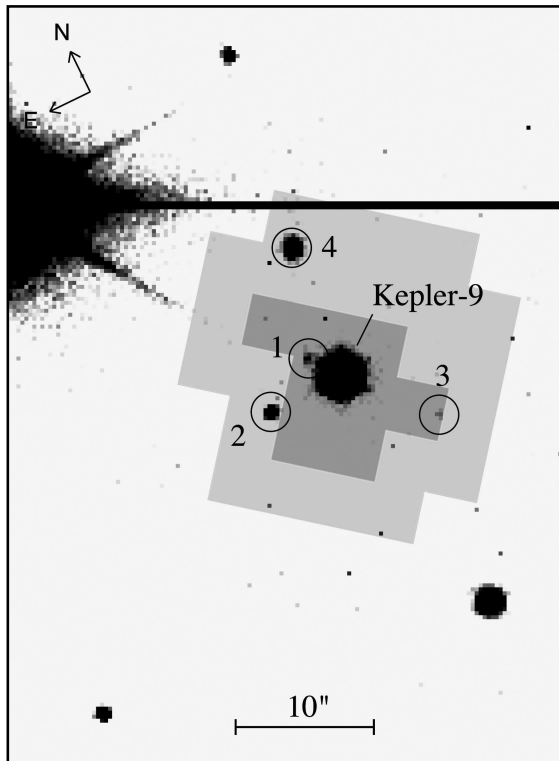
FIG. 1.— Image of Kepler-9 from the HIRES guider camera on the Keck I telescope, obtained in seeing of 0''.9 and clear skies. Companions within 15'' are labeled as in Table 1. The scale of the image is 0''.30 \text{ pix}^{-1} . Also indicated are the optimal photometric aperture (darker gray area of 8 pixels, used to extract the Kepler photometry) and the target aperture mask (lighter gray area of 31 pixels, used to measure centroids) for Kepler quarter 3.
