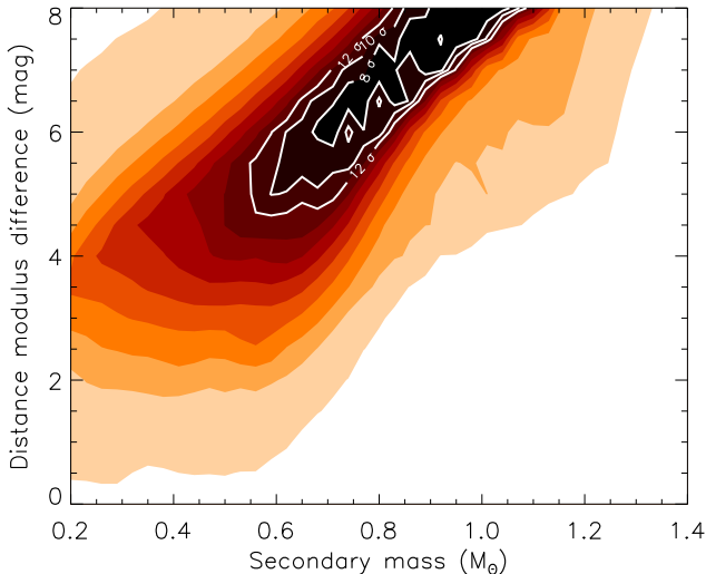
FIG. 15.— Same as Figure 10, but for the case in which the orbital period is assumed to be twice the nominal value ( 2P = 3.185702 days).
