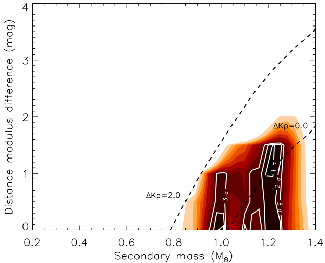
FIG. 9.— Same as Figure 6 (Kepler-9c), restricted to star-planet orbits having e = 0.3 (concentration of contours on the left) and 0.5 (right), and \omega = 90^\circ . This orientation corresponds to transits that occur at periastron. Comparison with Figure 6 shows that these solutions allow for more massive (larger) secondary stars than in the case of circular orbits, but the brightness of these blends is still within 2 magnitudes of the target, and is ruled out by spectroscopy.
