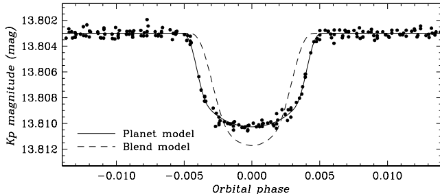
FIG. 4.— Light curve of Kepler-9b ( P = 19.24 days) with the best fit blend model for the case of a hierarchical triple (candidate + physically associated eclipsing binary). The best fit planet model is shown for reference. The poor fit of the blend model rules out this configuration.
