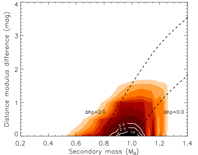
FIG. 6.— Map of the \chi^2 surface corresponding to a grid of blend models for Kepler-9c involving background eclipsing systems in which the tertiary is a (dark) planet, in a circular orbit around the secondary. Contours are labeled with the \chi^2 difference from the best planet model fit (expressed in units of the significance level of the difference, \sigma ). Two dashed lines of equal magnitude difference ( \Delta Kp ) are indicated, and show that all viable blend fits (with confidence level < 3\sigma ) have secondaries that are bright enough to have been detected spectroscopically ( \Delta Kp < 2 ).
