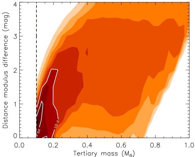
FIG. 5.— Map of the \chi^2 surface (goodness of fit) corresponding to a grid of blend models for Kepler-9c ( P = 38.91 days) involving background eclipsing binaries with circular orbits. The separation between the binary and the primary is expressed in terms of the distance modulus difference. Contours are labeled with the \chi^2 difference from the best planet model fit (expressed in units of the significance level of the difference, \sigma ), and are plotted here as a function of the mass of the tertiary star. The dashed line at 0.1 M_{\odot} indicates the lower limit to the tertiary mass set by the model isochrones we use.
