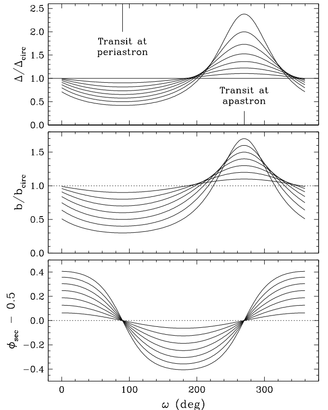
FIG. 8.— Effect of eccentricity on the duration of transits relative to the circular orbit case ( \Delta/\Delta_{\text{circ}} ), on the impact parameter ( b/b_{\text{circ}} ), and on the displacement ( \phi_{\text{sec}} - 0.5 ) of the secondary eclipses relative to phase 0.5, all shown as a function of the longitude of periastron \omega . The different curves correspond to eccentricities from 0.1 to 0.7 in steps of 0.1.
