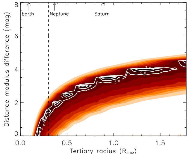
FIG. 14.— Same as Figure 13, shown here as a function of the tertiary radius. Kinks in the contours and closed inner contours for the 1\text{-}\sigma and 2\text{-}\sigma levels are an artifact of the discreteness of our grid. We indicate with a dashed line the lower limit for the size of the tertiaries that is set by the spectroscopic constraint on presence of bright stellar companions (see text). The size of the Earth, Neptune, and Saturn are also indicated for reference.
