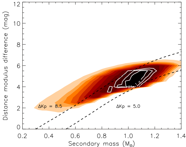
FIG. 12.— Same as Figure 10, including the effect of differential extinction in the amount of 0.5 \text{ mag kpc}^{-1} . The net effect of extinction is to compress and shift the contours toward smaller relative distances. The dashed lines indicate levels of equal apparent magnitude difference \Delta Kp between the background binary and the primary star, and are the same as shown in Figure 10.
