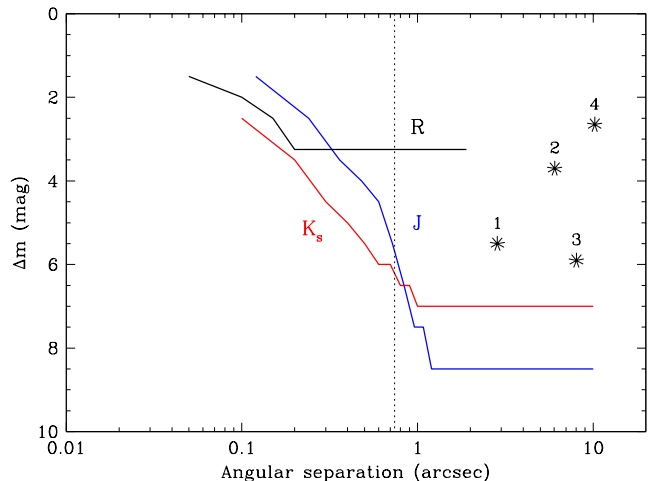
FIG. 2.— Sensitivity to faint companions near Kepler-9 from our imaging observations. Any companions above the curves are bright enough to be detected. J and K s limits are from AO observations at the Palomar 200-inch telescope, and R is from speckle observations using the WIYN 3.5 m telescope. Companions to the right of the vertical dotted line at 0''.74 cannot be responsible for the 1.6-day signal, as they would have induced centroid motion that is not observed. Stars detected in our imaging observations (Table 1) are marked with asterisks at their measured angular separations and magnitude differences in the Kepler passband.
