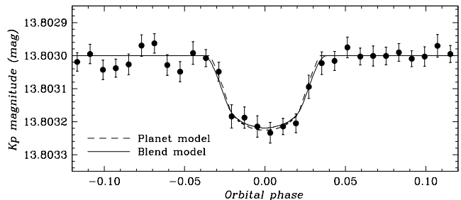
FIG. 11.— Example of a blend model fit to KOI-377.03 involving a background eclipsing binary with a stellar tertiary (solid line). The secondary is similar in spectral type to the primary and 5.2 mag dimmer, and the tertiary is a late M dwarf. The eclipsing pair is 6 kpc behind the primary. This fit is statistically indistinguishable from the best fit planet model, which is shown with a dashed line. The Kepler observations have been binned for clarity.
